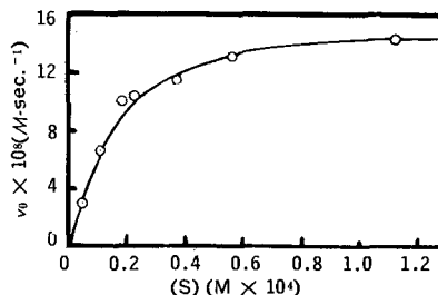
Fig. 2—Initial velocity against substrate concentration for the chymotrypsin-catalyzed hydrolysis of p -APT C ; pH = 7.05, [E]_0 = 4.02 \times 10^{-6} M.
